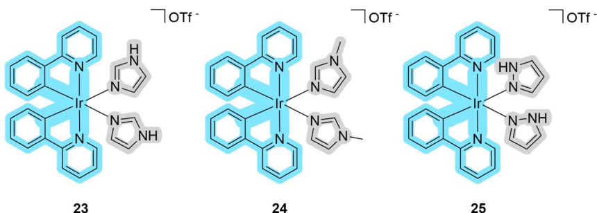
Fig. 8 Structures of iridium complexes 23–25 that exhibit properties of PDT/PACT agents. Blue indicates the part responsible for PDT, while gray indicates the released ligand.
