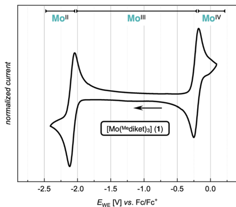
Fig. 2 CV of [Mo(Me Me diket) 3 ] ( 1 ) (1 mM) in TBAPF 6 /MeCN (0.1 M) at a scan rate of \nu = 100 mV s -1 .
