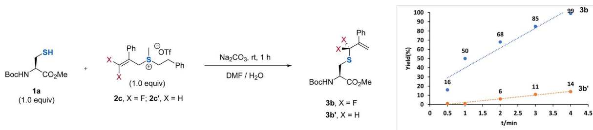
Fig. 2 Kinetic studies of the reaction of 1a with 2c or 2c' .
