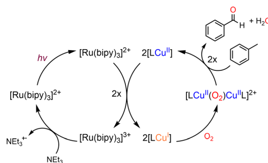
Scheme 12 Complex LCu(I) (L = tmpa (tris(2-pyridylmethyl)amine)) after reaction with \text{O}_2 according Göttlich and Schindler 206 and proposed general catalytic cycle for toluene oxidation (adapted from ref. 206).
