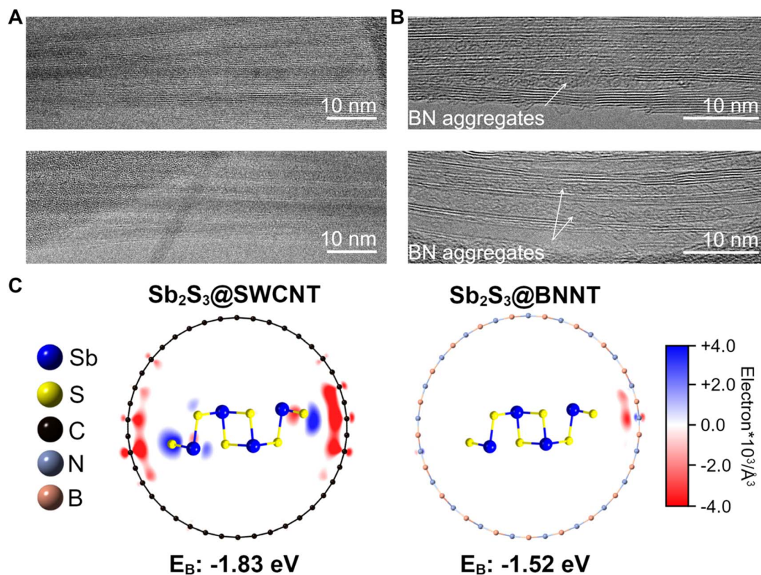
Fig. 4 HRTEM of \text{Sb}_2\text{S}_3@\text{BNNTs} and DFT simulations of \text{Sb}_2\text{S}_3@\text{nanotubes} . (A) Representative HRTEM image of amorphous \text{a-Sb}_2\text{S}_3 domains within apparently smooth and well-defined BNNTs. (B) Representative HRTEM images of BNNTs before filling with \text{Sb}_2\text{S}_3 . Highlighted in arrows are the BN aggregates that are encapsulated inside the nanotubes. (C) DFT and electron density difference map of crystalline \text{Sb}_2\text{S}_3 in a (21,0) SWCNT and (21,0) SBWNT.
