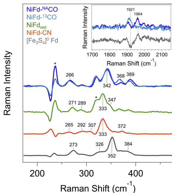
Fig. 4 Resonance Raman spectra of [\text{Fe}_3\text{S}_4]^0\text{Fd} (gray), NiFd red (green), NiFd-CN (orange), and NiFd-CO (blue). Samples were collected at 77\text{ K} using an excitation wavelength of 407\text{ nm} , P = 8\text{ mW} . Residual features corresponding to buffer are indicated with an *. Bands arising from buffer, DT, and quartz were subtracted after collection. (Inset) High frequency region of the resonance Raman spectra of NiFd-CO prepared with natural abundance CO (dark blue) and ^{13}\text{CO} (light blue), shown offset from the difference spectrum (gray). The band at 1906\text{ cm}^{-1} is present in both samples and independent of the CO isotope.
