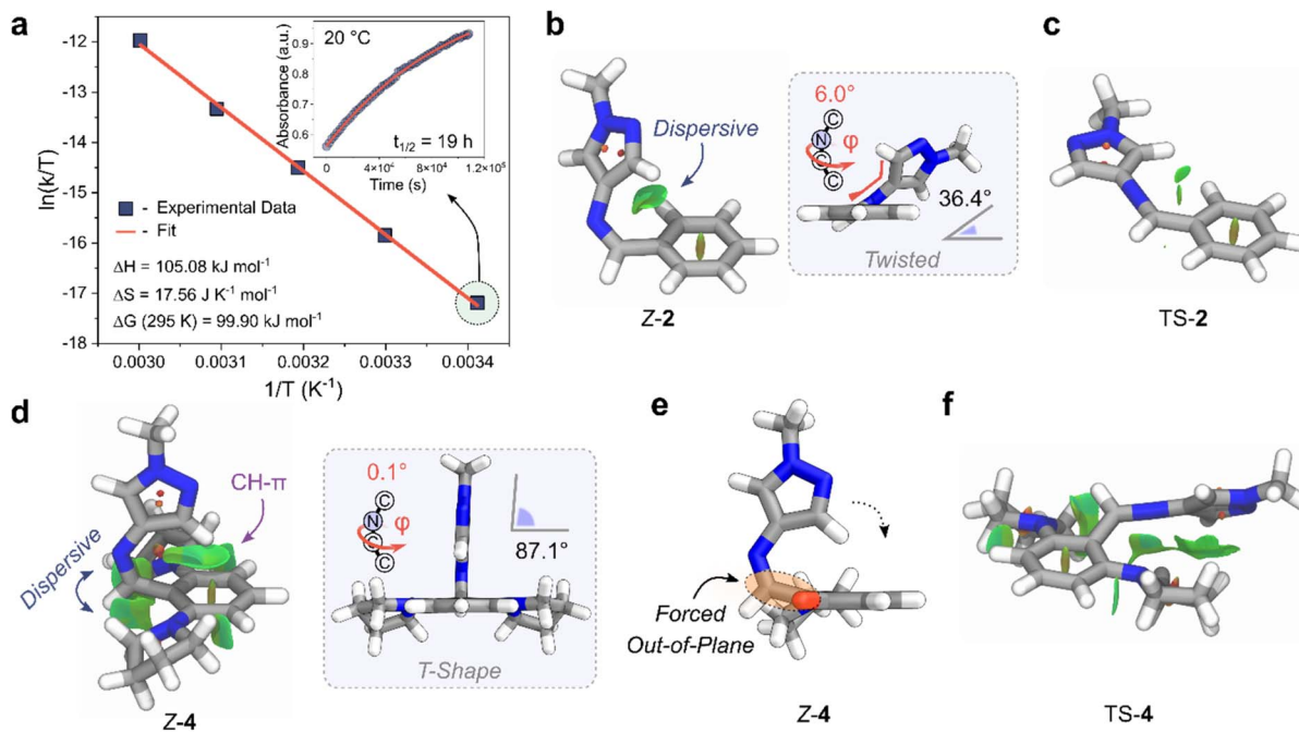
Fig. 5 (a) Eyring plot of the longest-lived Z-AIP, 4. (inset) Rate of thermal reversion of the Z-to-E isomer at 20^\circ\text{C} . (b) Geometry-optimized Z-2 highlighting green NCI surfaces between the pyrazole and phenyl rings. (inset) Display of the twisted geometry. (c) Geometry-optimized TS-2 with NCI surfaces displayed. (d) Geometry-optimized Z-4 showing large NCI interactions between the imine and the ortho -pyrrolidine units, as well as CH- \pi interactions between the CH of the pyrazole and the phenyl ring. (inset) View showing the T-Shape conformation. (e) Alternate view of Z-4; the pyrrolidine projecting out of the page is depicted as a red stub for clarity. (f) Geometry-optimized structure of TS-4 with NCI surfaces displayed.
