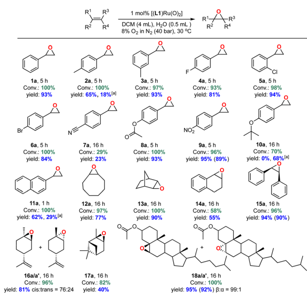
Fig. 13 Substrate scope of [(\mathbf{L1})\text{Ru}^{\text{VI}}(\text{O})_2(\text{H}_2\text{O})_2] catalysed aerobic alkene epoxidation. Conversions and yields determined by quantitative ^1\text{H} NMR spectroscopy against mesitylene as internal standard; isolated yields provided in parentheses. [a] Yield of corresponding aldehyde from epoxide isomerisation.
