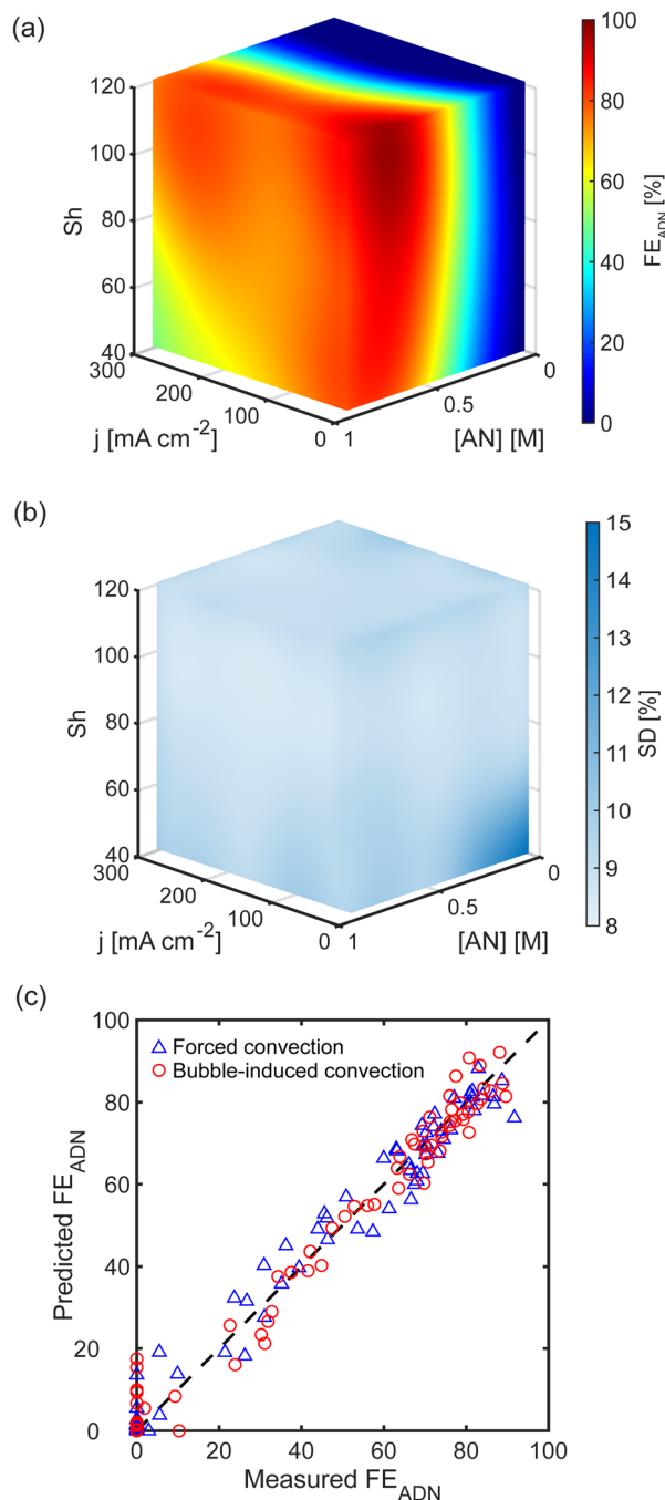
Fig. 7 Unified surrogate model performance. (a) 3D GPR unified surrogate model showing the effect of current density ( j ), AN concentration ([AN]), and Sherwood number (Sh) on FE_{ADN} . The unified model is built on the combined forced and bubble-induced convection experimental data. (b) Standard deviation (SD) of the surrogate model predictions. The average SD is 9.3% (absolute), and the largest standard deviations are at low j , low [AN], and low Sh, where FE_{ADN} is expected to be near zero. (c) The unified model predicted FE_{ADN} vs. measured FE_{ADN} from the forced and bubble-induced convection experiments. The predictions have an RMSE of 5.2% (absolute) compared to measured values. Reactions were performed at ambient temperature and pressure. In addition to AN, the electrolyte contained 0.5 M Na_3PO_4 , 0.03 M EDTA, and 0.02 M TBA hydroxide.
