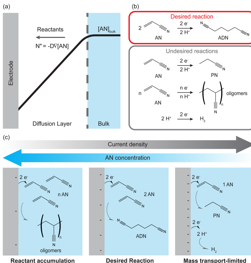
Fig. 1 (a) Schematic of mass transport limitations in electrochemical reactors. Reactants at bulk concentration [AN]_{bulk} are depleted at the electrode surface by electrochemical reactions (molar flux N'' = j/nF where j is the current density, n is the number of electrons involved in the reaction, and F is the Faraday constant). In mass transport limited reactions, the reaction rate is limited by the diffusion of reactants from the bulk to the electrode surface (diffusive flux: N'' = -D \nabla [AN] where D is the diffusivity). (b) Cathodic desired and undesired reactions in the electrohydrodimerization of acrylonitrile (AN) to adiponitrile (ADN). Competing reactions include the production of propionitrile (PN), AN-derived oligomers, and the hydrogen evolution reaction (HER). (c) Effect of mass transport limitations on product selectivity in the electrohydrodimerization of AN to ADN. Oligomers and polymers are favored at low current density and high AN concentration at the electrode. The desired reaction, ADN production, occurs at low current density and moderate AN concentration. At high current density, the AN concentration at the electrode is depleted, favoring PN production or hydrogen evolution.
