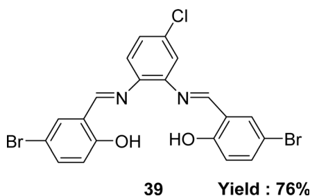
Fig. 22 Structure of Schiff base ligand 39.
