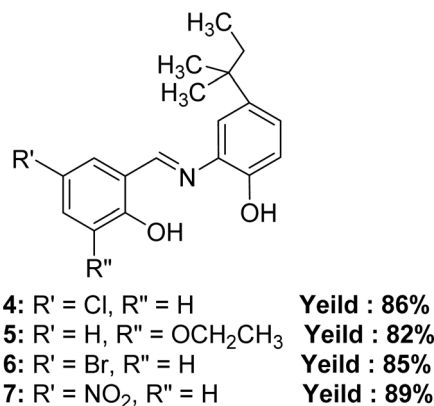
Fig. 15 Structure of Schiff base ligands 14, 15, 16 and 17.
