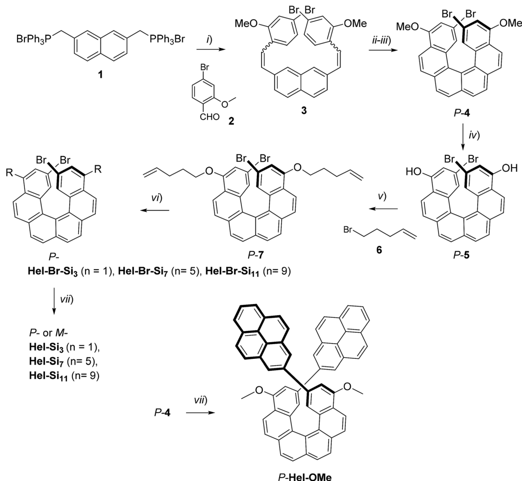
Scheme 1 Synthetic route to enantiopure oDMS end-functionalized carbo[6]helicenes P - Hel-Si 3 , Hel-Si 7 , Hel-Si 11 and Hel-OMe . (i) n -BuLi, rt, Ar, 3 h, 94%; (ii) I 2 , toluene, Ar, propylene oxide, hν , 7 h, 61%; (iii) chiral HPLC resolution (see the ESI†); (iv) BBr 3 , CH 2 Cl 2 , rt, Ar, 12 h; (v) K 2 CO 3 , DMF, Ar, 65 °C, overnight, 67%; (vi) Karstedt's catalyst, Si (2+n) H, CH 2 Cl 2 , rt, Ar, 12 h, 73% ( n = 1), 59% ( n = 5, 9); (vii) pyrene-2-boronic acid, Pd(PPh 3 ) 4 , Na 2 CO 3 , DMF, 80 °C, Ar, 12 h, 43–55%. The same strategy was used for the M enantiomers. The detailed R substituents can be seen in Fig. 1.
