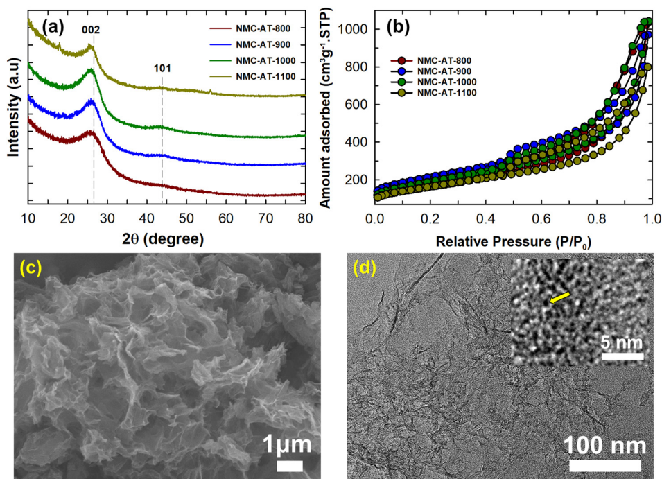
Fig. 2 (a) Powder X-ray diffraction patterns and (b) nitrogen adsorption–desorption isotherms of NMC-AT samples. (c) SEM image and (d) TEM image of the NMC-AT-1000 sample.
