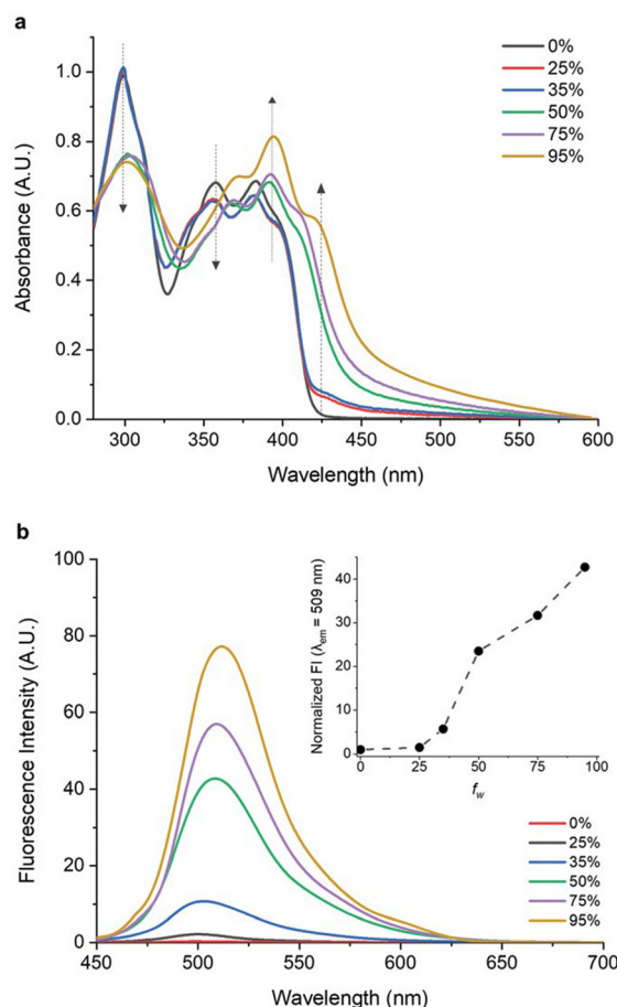
Fig. 4 (a) UV–vis spectra of dilute solutions of 16 in THF–H 2 O mixtures with different volume fractions of water ( f_w ). (b) PL spectra of 16 in THF–H 2 O mixtures at different fw values. The inset shows the normalized PL intensity at \lambda_{em} = 509 \text{ nm} as f_w changes. Partially reproduced with permission from ref. 55. Copyright 2021 Wiley.
