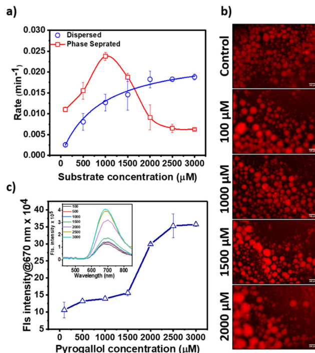
Fig. 2 (a) Kinetics of the oxidation of pyrogallol to purpurugallin catalysed by the BSA-Gold nanocluster (AuNC@BSA) in the presence of high excess \text{H}_2\text{O}_2 (0.1 M) in dispersed and phase separated (PS) conditions, (b) fluorescence microscopy images of Texas red labelled AuNC@BSA in the absence (control) and presence of different concentrations (100 \mu\text{M} , 1000 \mu\text{M} , 1500 \mu\text{M} and 2000 \mu\text{M} ) of pyrogallol. Images are taken after starting the oxidation reaction by the addition of \text{H}_2\text{O}_2 . Scale bar is 100 \mu\text{m} . (c) Change in fluorescence of AuNC@BSA with increasing concentration of pyrogallol.
