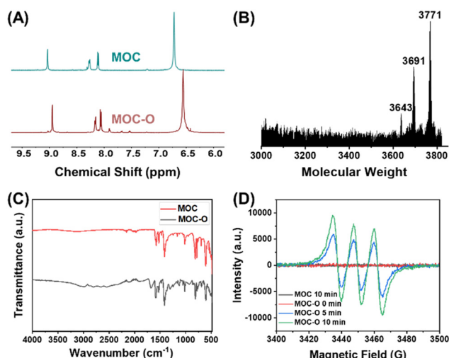
Fig. 1 The structural characterization of MOC and MOC-O nanozymes. (A) The 1 H-NMR spectra of the MOC and MOC-O in \text{DMSO-}d_6 . (B) The MALDI-TOF mass spectrum of MOC-O. (C) The FT-IR spectra of the MOC and MOC-O. (D) The EPR curves of the MOC and MOC-O.
