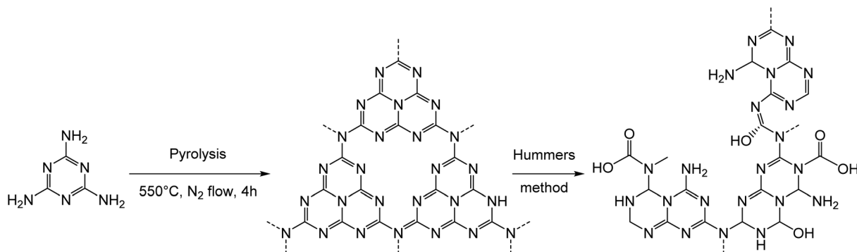
Scheme 2 Synthesis and proposed structure of oxCN Mel- .
