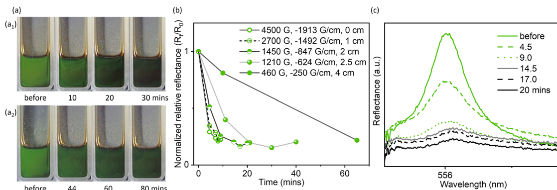
Fig. 3 (a) Photographs of the green hydrophobic GO- \text{Fe}_3\text{O}_4 photonic liquids (mass ratio, \sim 1:1 ; in butyl acetate) in response to decreasing magnetic fields at different times (1450 G for a 1 and 460 G for a 2 ). (b) Normalized relative reflectance of the GO- \text{Fe}_3\text{O}_4 photonic liquids in response to field strength at different times. (c) Reflection spectra of the green hydrophobic GO- \text{Fe}_3\text{O}_4 photonic liquids shown in a 1 in response to a 1450 G magnetic field with increasing time. The magnet was positioned behind the samples.
