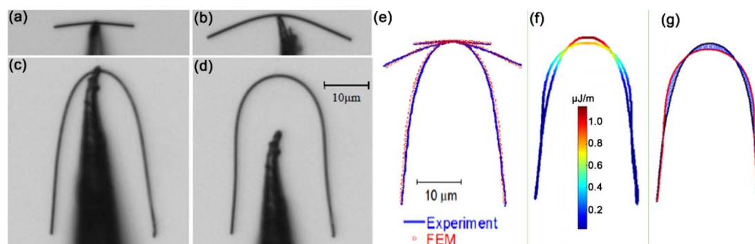
Fig. 25 (a–c) Optical micrographs of three NW segments with difference lengths pushed to slide along the Si substrate by a W tip. (d) Optical micrograph of the NW shown in (c) after tip removal. (e) The comparison of NW profiles before tip removal from the tests and the FEM simulations. (f) Distribution of elastic energies per unit length of the bent NW shown in (c) and (d), and (g) the corresponding the swept area A_{\text{swept}} (crossed). Reproduced with permission. 219 Copyright 2016, IOP.
