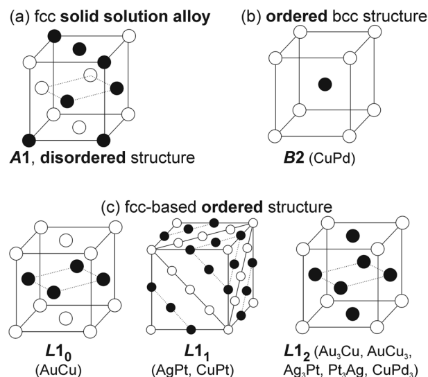
Fig. 5 Crystal structures of (a) SSAs and some (b) and (c) intermetallics of B2, L1_0 , L1_1 , and L1_2 -typed ordered structures.
