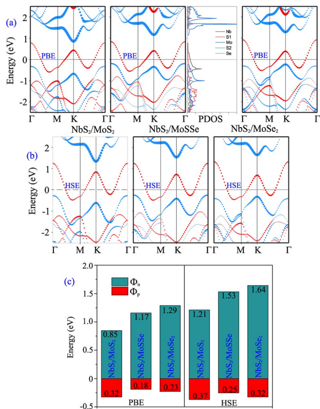
Fig. 4 Projected band structures of NbS 2 /MoS 2 , NbS 2 /MoSe and NbS 2 /MoSe 2 heterostructures obtained using (a) PBE and (b) HSE functionals. (c) Schottky barriers of NbS 2 /MoS 2 , NbS 2 /MoSe and NbS 2 /MoSe 2 heterostructures for the most energetically stable AB3 configuration. The inset presents the partial density of states (PDOS) of all atoms in the NbS 2 /MoSe heterostructure for the AB3 stacking configuration.
