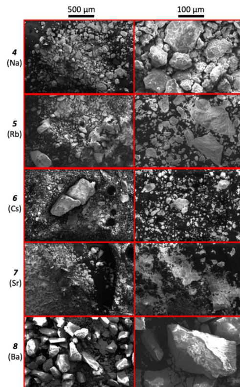
Fig. 7 SEM micrographs at 100× (left, scale: 500 μm) and 500× (right, scale: 100 μm) magnification of 4 (Na) to 8 (Ba).
