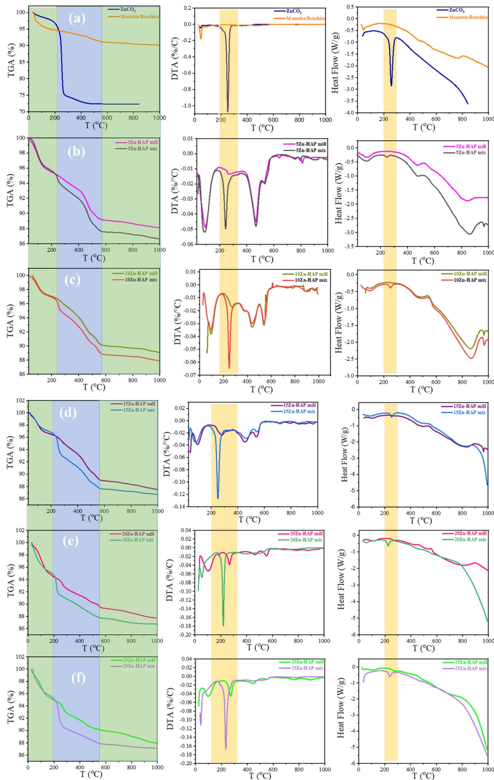
Fig. 5 TGA (left), DTA (middle), and DSC (right) for (a) ZnCO 3 and monetite/brushite, (b) 5 Zn-HAP mill and 5 Zn-HAP mix, (c) 10 Zn-HAP mill and 10 Zn-HAP mix, (d) 15 Zn-HAP mill and 15 Zn-HAP mix, (e) 20 Zn-HAP mill and 20 Zn-HAP mix, and (f) 25 Zn-HAP mill and 25 Zn-HAP mix.
