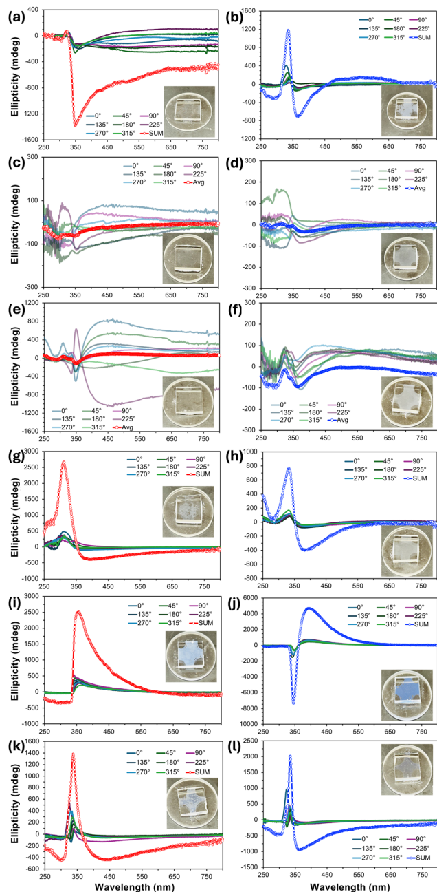
Fig. 5 Thin-film CD spectra taken at 45° sample rotation angles ( \Delta\epsilon [mdeg] vs. \lambda [nm]) of 10- \mu\text{m} films between untreated quartz substrates after cooling at a different rate from the isotropic liquid phase to room temperature ( T \sim 20^\circ\text{C} ) at different sample rotation angles as indicated in the legends (red SUM or average (Avg) datasets to cancel out linear dichroism and birefringence are for slow cooling ( <5^\circ\text{C min}^{-1} ); blue SUM or Avg datasets for rapid cooling ( \geq 50^\circ\text{C min}^{-1} )): (a) and (b) BC1 , (c) and (d) BC2 , (e) and (f) BC3 , (g) and (h) BC4 , (i) and (j) BC5 , and (k) and (l) BC6 . Insets in each graph are the sample photographs either showing or lacking blue structural color. Average rather than SUM spectra were generated from the individual 45° sample rotation datasets when the resulting graphs showed randomly positive or negative weaker signals over broader or specific spectral ranges (i.e., for BC2 and BC3 ).
