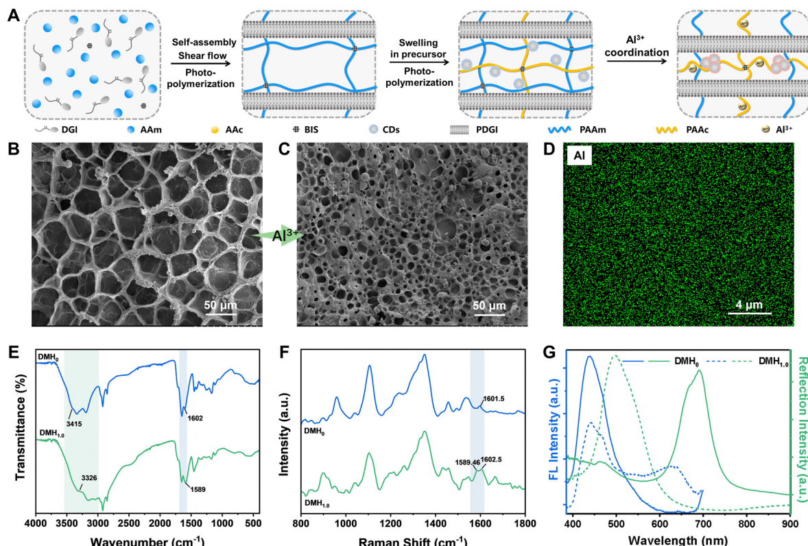
Fig. 1 Preparation and characterization of dual-mode hydrogels with or without \text{Al}^{3+} ions. (A) The flow chart of preparing dual-mode hydrogels and the coordination process with \text{Al}^{3+} ions. (B) and (C) SEM images of pDGI-PAAm/P(AAc-CDs) hydrogel before and after coordinating with \text{Al}^{3+} ions. (D) EDS mapping of Al in pDGI-PAAm/P(AAc-CDs) after being treated with \text{Al}^{3+} solution. (E) ATR-FTIR spectra and (F) Raman spectra of pDGI-PAAm/P(AAc-CDs) hydrogel before and after coordinating with \text{Al}^{3+} . (G) Fluorescence spectra ( \lambda_{\text{ex}} = 365\ \text{nm} ) and reflection spectra of the dual-mode hydrogel before and after coordinating with \text{Al}^{3+} .
