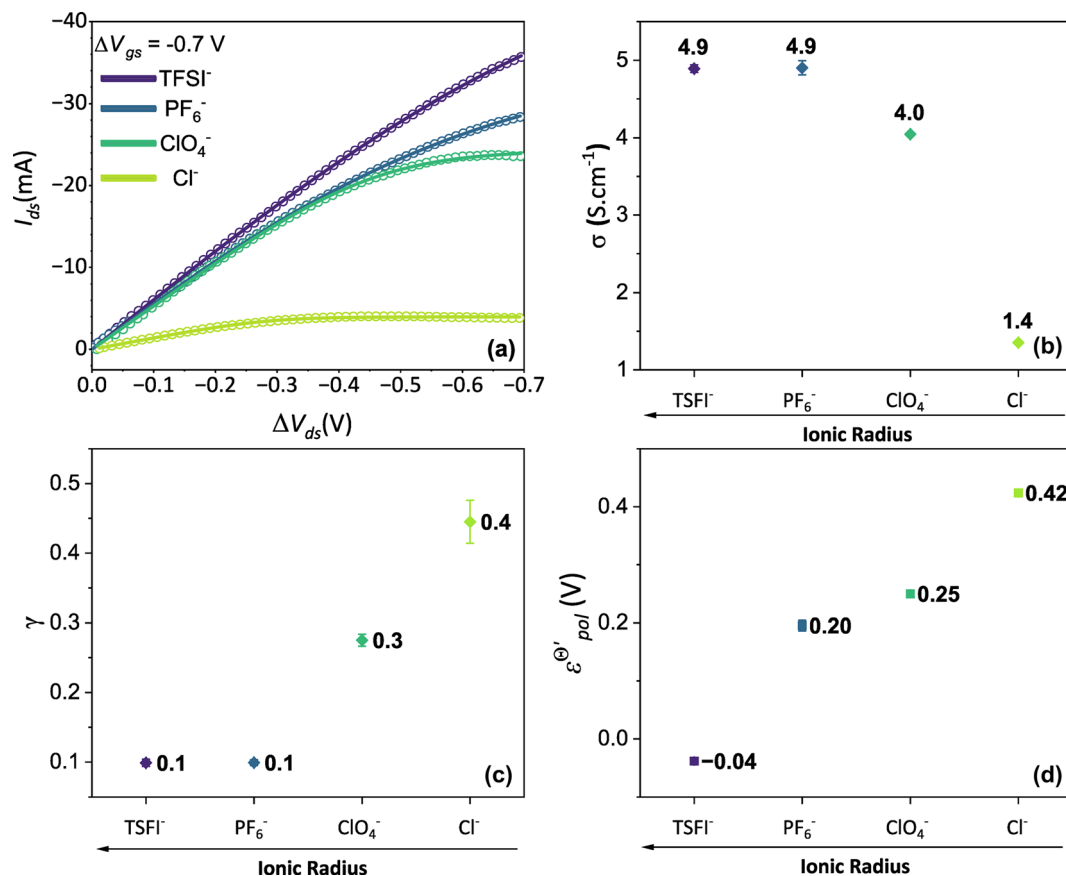
Fig. 5 (a) Output curves (hollow circles) from Flagg (2018), and fitting curves (solid lines) (b) \sigma , (c) \gamma and (d) \varepsilon_{\text{pol}}' parameters. Reprinted (adapted) with permission from Flagg et al. (2018). 26 Copyright © 2018, American Chemical Society. All data fittings with R^2 = 0.99 and p -values < 0.05 .
