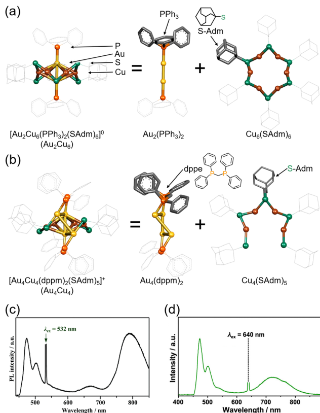
Fig. 17 (a) Schematic illustration of Au_2Cu_6 . (b) Schematic illustration of Au_4Cu_4 . (c) Photoluminescence spectrum obtained for the deaerated solution of Au_2Cu_6 /perylene with the 532 nm CW laser excitation. Reproduced from ref. 110 with permission from Royal Society of Chemistry, Copyright 2022. (d) Photoluminescence spectrum obtained for the deaerated solution of Au_4Cu_4 /perylene with the 640 nm CW laser excitation. Reproduced from ref. 112 with permission from American Chemical Society, Copyright 2023.
