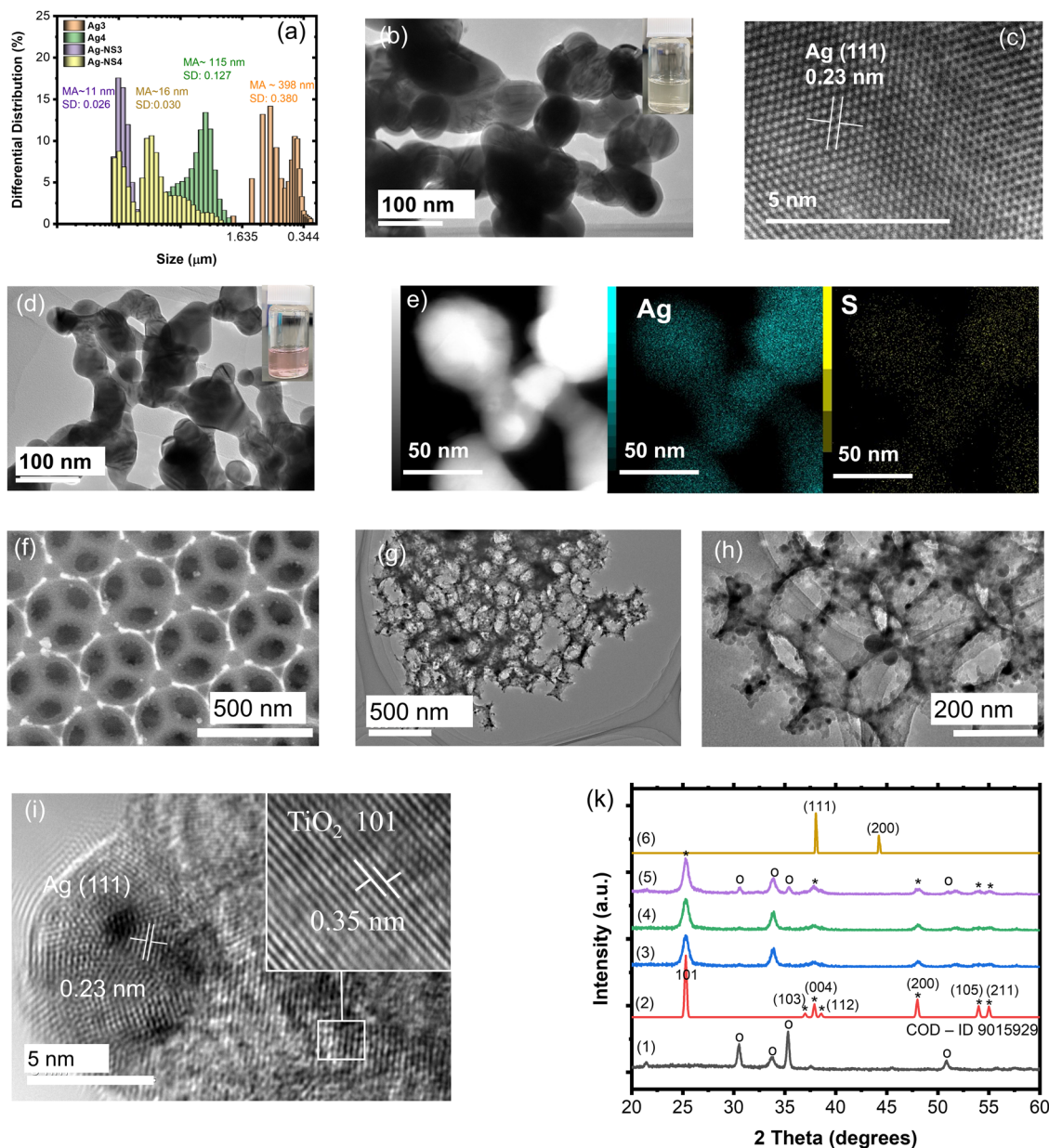
Fig. 3 (a) Differential distribution and size distributions of the Ag 3 , Ag 4 , AgNS 3 , and AgNS 4 NPs after synthesizing for 1 hour. (b) and (c) HR-TEM images of Ag 4 NPs. (d) HR-TEM images and (e) STEM-EDX mapping of element compositions of AgNS 4 NPs. (f) SEM and (g)–(i) HR-TEM images of TiO 2 deposited AgNS 4 at different magnifications. (k) XRD pattern of the ITO-coated glass (1), anatase TiO 2 (reproduced using a file with COD-ID 9015929) (2), TiO 2 50 (3), Ag 4 deposited TiO 2 50 (4), AgNS 4 deposited TiO 2 50 (5) and Ag 4 NPs (6). *Photograph of the Ag 4 and AgNS 4 NPs associated in methanol.
