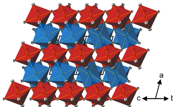
Fig. 4 Projection of the dirutile-type crystal structure of \text{CoTeO}_4 along [011] . [\text{CoO}_6] octahedra are given in blue, [\text{TeO}_6] octahedra in red. Displacement ellipsoids are drawn at the 90% probability level.
