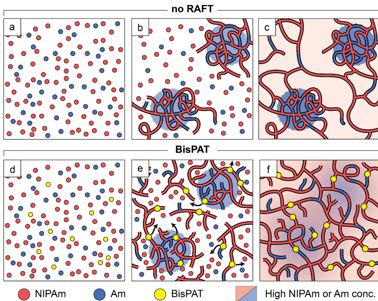
Fig. 4 Schematic of network copolymer formation in the no-RAFT and BisPAT PE 3D printing systems. (a) No-RAFT starting materials form: (b) high crosslink density nanogels in the early stages of the reaction that are rich in Am due to the NIPAm–Am reactivity ratios; (c) later in the no-RAFT reaction the nanogels are crosslinked with the resulting copolymer chains showing a higher relative NIPAm composition. (d) Starting materials in the systems containing BisPAT: (e) form more highly branched polymer chains prior to gelation which still contain a high Am content, but also contain trithiocarbonate units within the main chains; (f) further reaction and degenerative chain transfer allows the main chains to fragment and react further with NIPAm in the later stages of the reaction. The relaxation of the Am rich copolymer chains effectively increases the homogeneity of the Am–NIPAm composition throughout the network.
