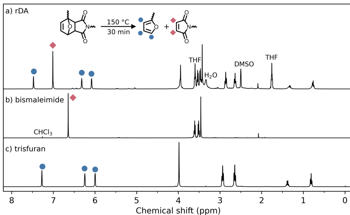
Fig. 5 ^1\text{H-NMR} spectra of (a) the DA-adduct after 30 minutes at 150 °C in DMSO- d_6 , (b) the bismaleimide monomer recorded in CDCl 3 and (c) the trisfuran monomer recorded in CDCl 3 . The THF observed in spectrum (a) is attributed to residual THF after the swelling tests.
