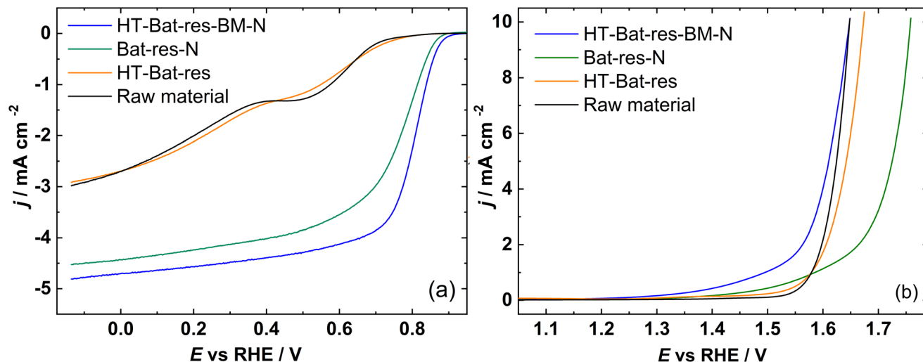
Fig. 3 RDE electrochemical characteristics of the studied materials: (a) ORR polarization curves at 1600 rpm in \text{O}_2 -saturated 0.1 M KOH solution and (b) OER polarization curves at 1600 rpm in \text{N}_2 -saturated 1 M KOH solution.
