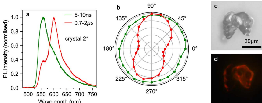
Fig. 6 Origins of anomalous photoluminescence behaviour of rubrene crystals. (a) Normalised PL spectra from crystal 2*, gated from 5–10 ns (green) and 0.7–2 \mu s (red). (b) The dependence of PL intensity (at 565 nm, green and 607 nm, red) on detection polariser angle for the two spectra shown in (a). (c) Microscope image of a microcrystal defect on the surface of crystal 2. Such a defect is a candidate source of the emission from crystal 2*. (d) Image of the photoluminescence from the defect shown in (c). The defect is much brighter than the bulk crystal.
