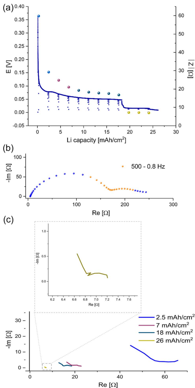
Fig. 4 (a) The voltage trace ( E-t ) of galvanostatic plating a total of 26 \text{ mA h cm}^{-2} Li at 1 \text{ mA cm}^{-2} in Li symmetric cell with LP30 electrolyte and GF separator at RT. EIS module values (spheres) were measured with GEIS at 9 Hz with 100 \mu\text{A} amplitude at 500–0.8 Hz. (b) A Nyquist plot of the PEIS spectrum of a symmetric lithium cell, LP30 electrolyte with GF separator measured after native SEI formation and before Li plating with 10 \text{ mV} amplitude at RT. The frequency range used in the following GEIS measurements is indicated in orange. (c) Nyquist plots measured with GEIS, 100 \mu\text{A} amplitude at RT during Li plating in a symmetric cell, LP30 electrolyte RT with GF separator. Magnification of the plot measured after plating 26 \text{ mA h cm}^{-2} Li.
