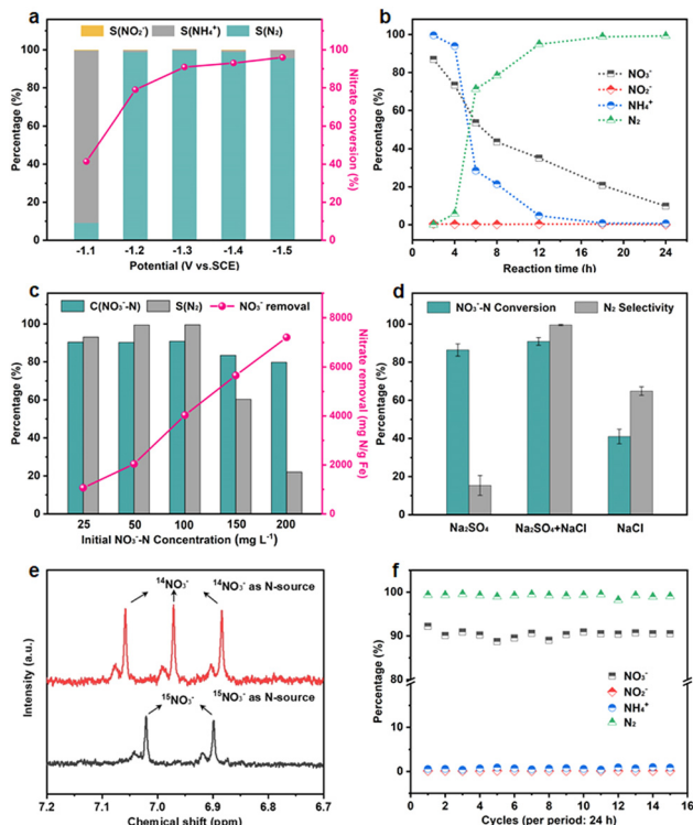
Fig. 4 (a) Nitrate conversion and product selectivity of \text{Fe}_3\text{C}/\text{MNCFs} -800 at different given potentials. (b) The evolution of \text{NO}_3^- , \text{NO}_2^- , \text{NH}_4^+ , and \text{N}_2 of \text{Fe}_3\text{C}/\text{MNCFs} -800 for different reaction times. (c) Nitrate conversion, \text{N}_2 selectivity, and nitrate removal capacity of \text{Fe}_3\text{C}/\text{MNCFs} -800 at different initial \text{NO}_3^- -N concentrations. (d) Nitrate conversion and \text{N}_2 selectivity of \text{Fe}_3\text{C}/\text{MNCFs} -800 at different electrolytes. (e) ^1\text{H} NMR spectra of the electrolyte after the electrocatalytic \text{NO}_3\text{RR} using ^{14}\text{NO}_3^- and ^{15}\text{NO}_3^- as the nitrogen source. (f) Nitrate conversion and \text{N}_2 selectivity of \text{Fe}_3\text{C}/\text{MNCFs} -800 during 15 consecutive cycles. Reaction conditions: 0.1 M \text{Na}_2\text{SO}_4 , 0.02 M NaCl, and -1.3 V, 24 h.
