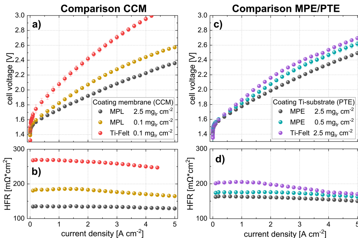
Fig. 8 Polarization curves and HFR measurements of selected measurements with MPLs and benchmarks using commercial Ti-felt materials from Bekaert (N115, T = 80 ^{\circ}\text{C} , 10 bar balanced pressure) using MPLs (a) and (b) CCM configuration and (c) and (d) MPE/PTE configuration all having an equal Pt-coating of 40 nm.
