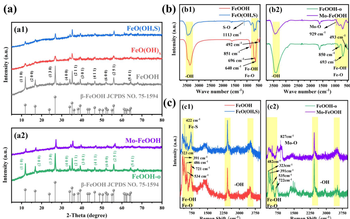
Fig. 1 (a) XRD patterns of different \text{FeOOH} samples: (a 1 ) pristine \text{FeOOH} and \text{FeO}(\text{OH}, \text{S}) catalysts; (a 2 ) \text{FeOOH-o} and \text{Mo-FeOOH(5%)} catalysts; (b) FTIR spectra of different \text{FeOOH} samples: (b 1 ) pristine \text{FeOOH} and \text{FeO}(\text{OH}, \text{S}) catalysts; (b 2 ) \text{FeOOH-o} and \text{Mo-FeOOH(5%)} catalysts; (c) Raman spectra of different \text{FeOOH} samples: (c 1 ) pristine \text{FeOOH} and \text{FeO}(\text{OH}, \text{S}) catalysts; (c 2 ) \text{FeOOH-o} and \text{Mo-FeOOH(5%)} catalysts.
