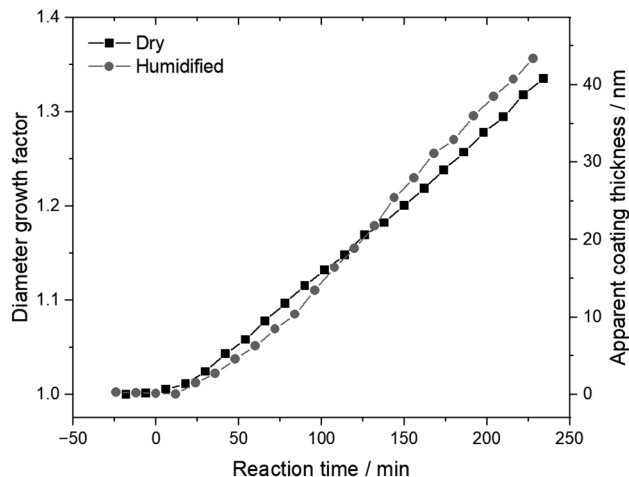
Fig. 1 Diameter growth factor and apparent coating thickness as functions of reaction time in the smog chamber for a representative experiment with initially 250 nm nanoplastics.
