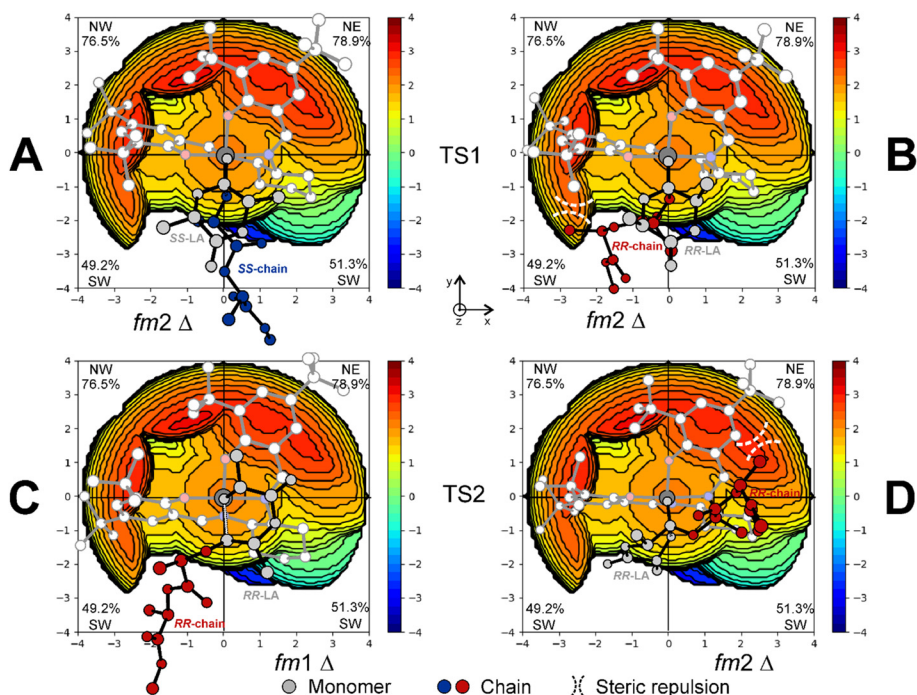
Fig. 7 % V_{\text{Bur}} steric maps of the RLS corresponding to TS1 for SS -LA (A) and RR -LA (B) propagations with catalyst ( R,R )-2A. Steric interactions leading to the TS2 preference for fm1 (C) vs. fm2 (D) for RR -LA propagation are reported with dashed lines. The z-axis is perpendicular to the plane containing the map.
