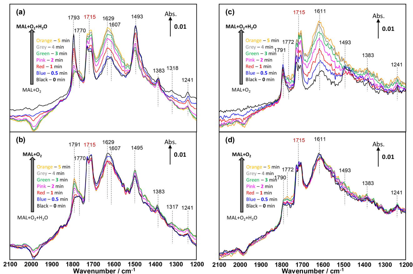
Fig. 7 Changes in in situ DRIFT spectra (2100–1200 \text{cm}^{-1} ) corresponding to the formation of MAA formation shown in Fig. 3 as a function of time on stream over HPmo (a and b) and HPmoV (c and d) catalysts at 320 °C during the 2nd cycle of switches of \text{H}_2\text{O} in and out of the MAL + \text{O}_2 gas feed. The gas feed is composed of 3500 ppm MAL, 7000 ppm \text{O}_2 , 7000 ppm \text{H}_2\text{O} (when added), and Ar balance and the total flow rate is 100 \text{cm}^3 \text{min}^{-1} .
