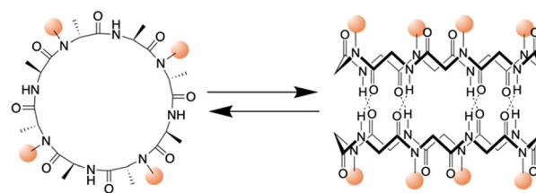
Fig. 3 Schematic illustration of the chemical structure of a cyclic peptide with N -methylated amino acids and the cylindrical dimeric ensemble.
