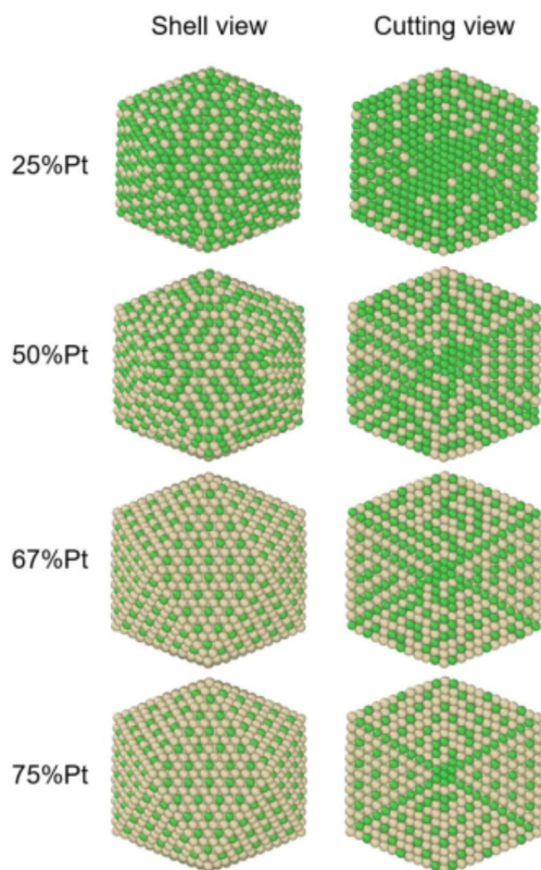
Fig. 10 Snapshots of Ih_{5083} NPs at different compositions and after thermal equilibration at 300 K, showing the chemical ordering from a shell view (left column) and a cutting view (right column). Green atoms represent Ni and beige atoms represent Pt.
