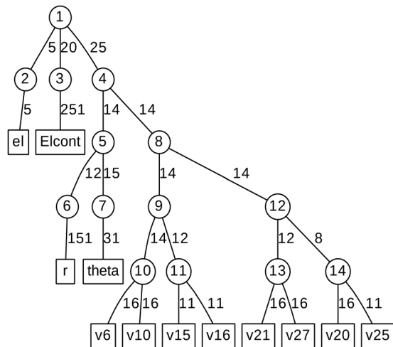
Fig. 3 Diagrammatic representation of the ML-MCTDH wavefunction. The circle represents a node on each layer and the square represents primitive bases or grids. 'el' indicates electronic degrees of freedom, 'Elcont' indicates the electronic continuum, 'r' indicates O–H bond stretch, 'theta' indicates C–C–O–H bond torsion, and 'v x ' indicates the vibrational normal modes (see text for details).
