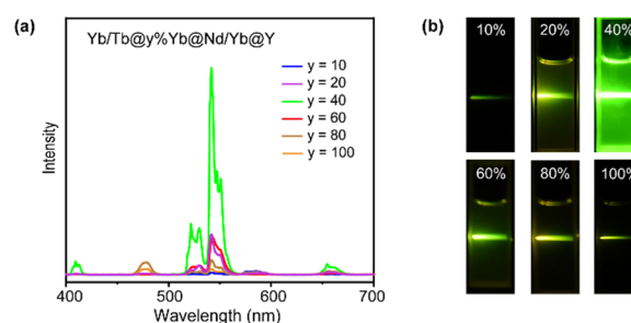
Fig. 3 (a) Upconversion luminescence spectra of \text{Tb}/\text{Yb}@y\%\text{Yb}@m\%\text{Nd}/m\%\text{Yb}@m\%\text{Y} CSSS NPs. (b) Digital photos of \text{Tb}/\text{Yb}@y\%\text{Yb}@m\%\text{Nd}/m\%\text{Yb}@m\%\text{Y} CSSS NPs.
