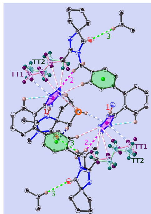
Fig. 2 View of the dimer in 1-A , at T = 130 \text{ K} and along [001] . Shown are the principal interactions (see Tables 1 and S8†) and the centre of inversion (red circle): N–H...N (red, u_1 ), C–H...O (green, u_3 ), C–H...N (pink, u_2 ), C–H... \pi (blue) and intramolecular bonds are turquoise. COG0 (pink) is the centre of gravity of the tetrazole, and COG1 (green) is that of the phenyl C1B,...,C6B. The all- trans n.b.c. TT1 is purple, and TT2 is blue-green (more complete figure in Fig. S64†).
