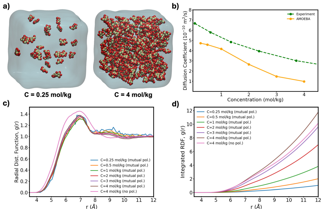
Fig. 4 (a) Lowest and highest Glc concentration modeled here. (b) Diffusion coefficient computed from eqn (1) as a function of concentration for our box sizes of \sim 60^3 \text{ Å}^3 ( \sim 20 k atoms). Extrapolation of MD-calculated diffusion coefficients to bulk conditions can yield a 10% increase 20 although no correction has been applied here. (c) Radial distribution function of the COM of \beta -Glc and (d) corresponding integration data.
