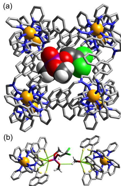
Fig. 2 Crystal structure of the \text{H}^\bullet -dichlorvos complex. (a) A view of the complete cage with the guest shown in space-filling mode; (b) a view of the guest (plus a MeOH molecule) emphasising the \text{CH}\cdots\text{O} interactions with the cage interior surface (green dotted lines).
