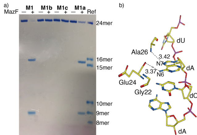
Fig. 3 (a) MazF-mediated cleavage of native ( M1 ) and 14 C, 3 H or 6 LiA modified RNA substrates ( M1a , M1b or M1c , respectively). The gel was stained by stain-all overnight and de-stained in MilliQ water. The reference sequences, of known length, are the following: 16-mer oligomer: 5'-ACA AUU CAG CUA UGC-3', 15-mer oligomer: 5'-ACA AUU CAG CUA UGC-3', 10-mer oligomer: 5'-GUA UAG CCA A-3', 9-mer oligomer: 5'-GUA UAG CCA-3', 8-mer oligomer: 5'-GUA UAG CC-3'. (b) X-Ray co-crystal structure of MazF and d(ACAU), a DNA substrate analogue, illustrating the contacts between the nucleobases and the protein backbone. (PDB ID code: 5CR2)
