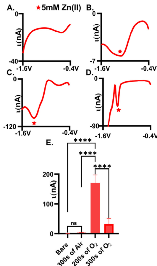
Fig. 1 Plasma treatment with oxygen positively impacts the detection of \text{Zn(II)} at AuMEs. Measurements were made using 5\text{ mM} \text{Zn(II)} in 1\text{ M} KCl. (A) No observable reduction peak at untreated gold fibers. (B) Minimal reduction current is observed on air plasma treated fibers at -1.3\text{ V} . (C) A clear reduction peak at -1.4\text{ V} is observed for \text{Zn(II)} at oxygen plasma treated gold fibers (treatment was for 200\text{ s} ). (D) Longer treatment times with oxygen plasma ( 300\text{ s} ) resulted in less observable current for \text{Zn(II)} reduction. (E) Comparison of treatments shows an overall 442\text{-fold} ( \sim 170.5\text{ nA} after treatment vs. 0.385\text{ nA} before treatment) increase for the detection of \text{Zn(II)} with 200\text{ s} of oxygen plasma treatment ( n = 6 ).
