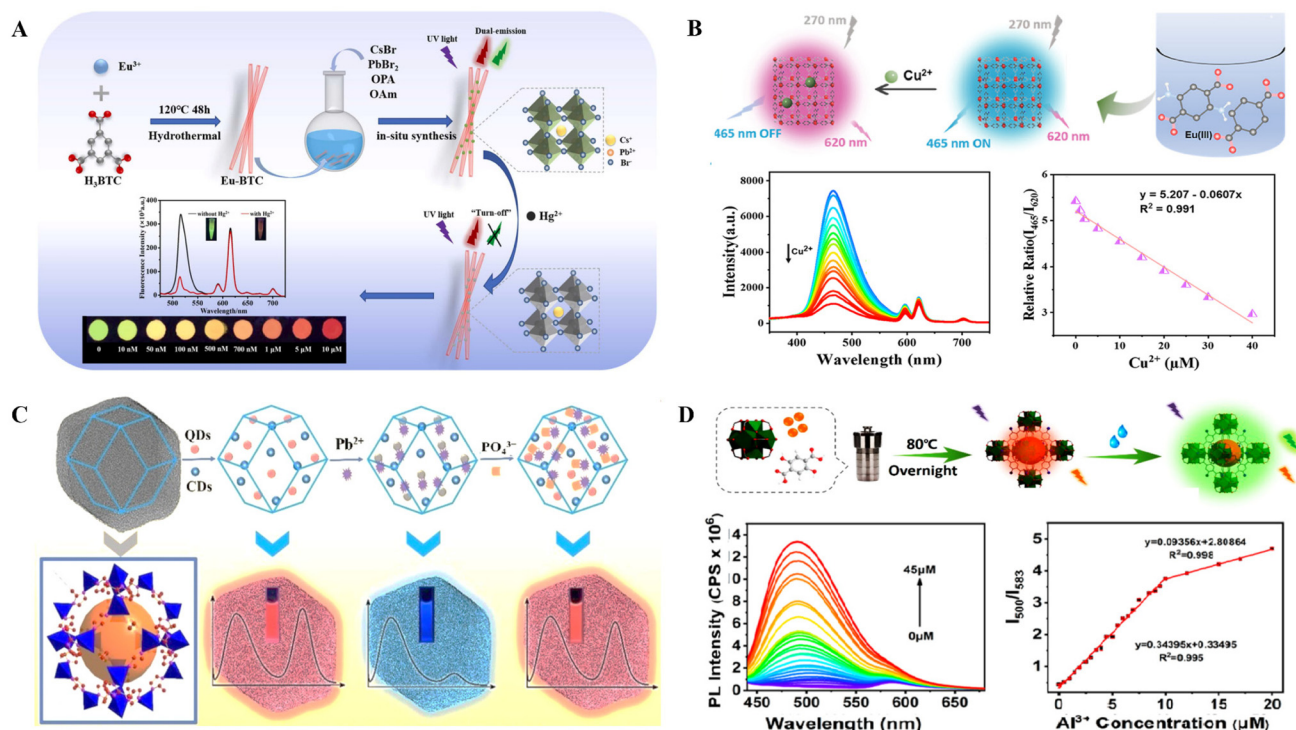
Fig. 7 Ion sensing of MOF-based ratiometric fluorescent probes. (A) Schematic diagram of the synthesis process of \text{CsPbBr}_3@Eu\text{-BTC} and the ratiometric fluorescence sensing of \text{Hg}^{2+} . 77 (B) Schematic diagram of ratiometric fluorescence sensing of \text{Cu}^{2+} in serum by \text{Eu-DATA/BDC} . 78 (C) Schematic diagram of \text{CDs/QDs@ZIF-8} for ratiometric fluorescence sensing of \text{Pb}^{2+} and \text{PO}_4^{3-} . 79 (D) Schematic diagram of the preparation of \text{UiO(OH)}_2@RhB and the sensing process for \text{Al}^{3+} . 80
