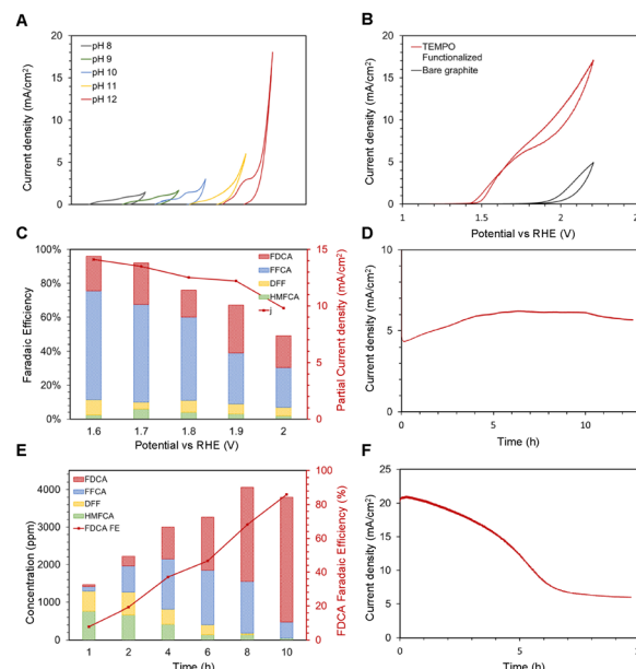
Fig. 5 (A) Cyclic voltammetry (CV) of TEMPO functionalized graphite in different pH electrolytes from pH 8 to pH 12. (B) Cyclic voltammetry of the TEMPO-immobilized graphite electrode (red) and the naked graphite electrode (black). Electrolyte conditions are 10 mM HMF and pH 12 electrolyte. (C) Faradaic efficiencies for each HMFOR product of immobilized TEMPO at various applied potentials. The partial current density is shown on the secondary y-axis, and balance FE is assumed to be the OER. (D) Chronoamperometry of TEMPO-GCE in 10 mM HMF and pH 12 electrolyte, at applied potential 1.7 V vs. RHE. (E) Product distribution over time of complete oxidation of 30 mM HMF, 1.7V vs. RHE. (F) Chronoamperometry of the complete oxidation experiment.
